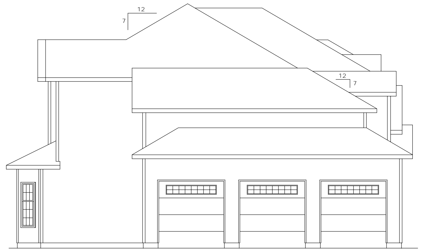
LEFT ELEVATION
